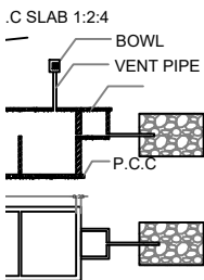
K AND TRENCH NTS
