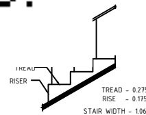
STAIRCASE DETAILS NTS
