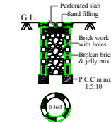
PERCOLATION PIT (NOT FOR SCALE)
