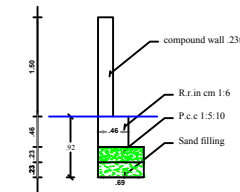
Compound Wall Detail
