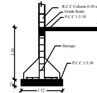
Column Detail
