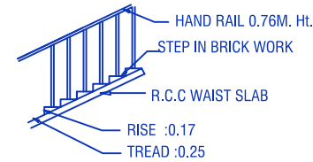
STAIR CASE DETAIL
