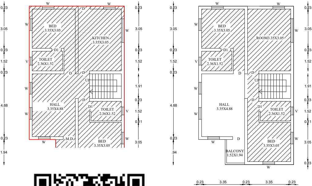
EXG FIRST FLOOR PLAN PRO FIRST FLOOR PLAN
