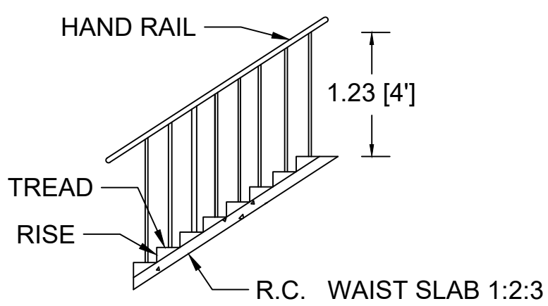
STAIRCASE DETAILS
