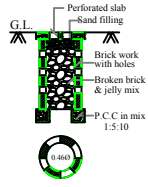
PERCOLATION PIT (NOT FOR SCALE)
