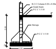
Column Detail
