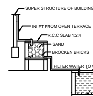
DETAILS OF FILTER BED & WELL
