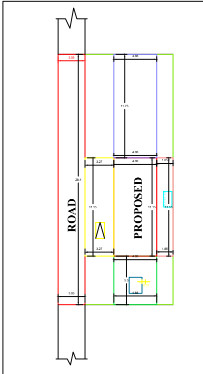
SITE PLAN
