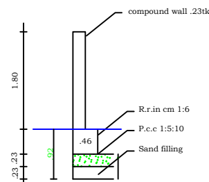
Compound wall Detail SCALE : (1:50)
