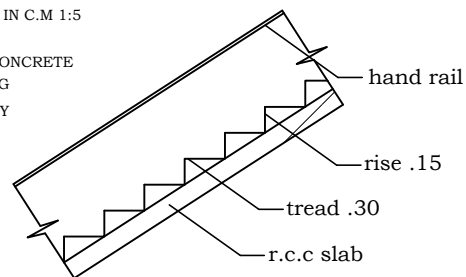
STAIR
