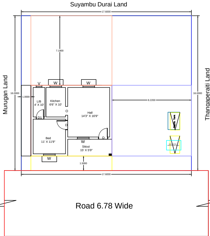
SEPTIC TANK AND TRENCH
