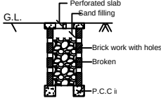
RAINWATER HARVESTING
