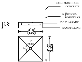
FOUNDATION DETAIL
