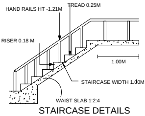
STAIRCASE DETAILS
