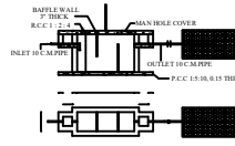
Baffle Wall & Cover
