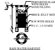
RAIN WATER HARVEST
