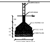
COLUMN DETAILS
