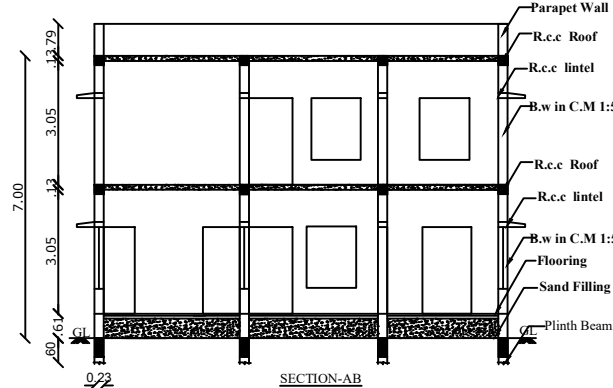
SECTION-AB
