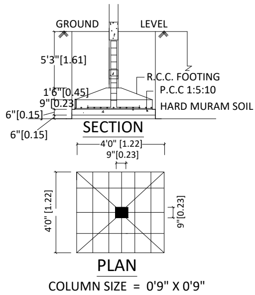
FOUNDATION DETAILS
