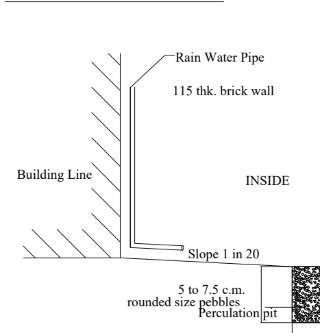
PERCOLATION PIT
