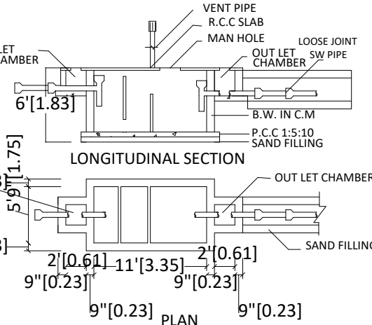
SEPTIC TANK:
