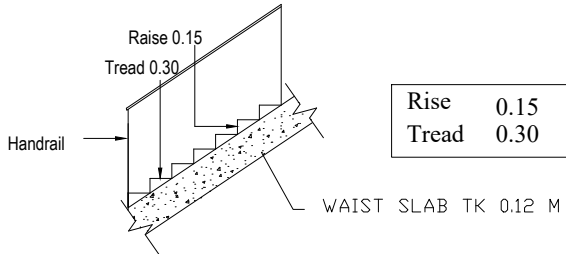
STAIRCASE DETAIL
