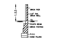
COMPOUND WALL DETAIL
