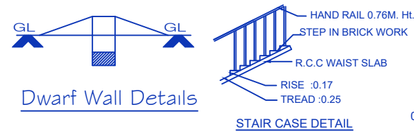
STAIR CASE DETAIL
