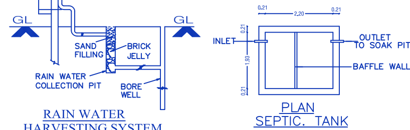
SECTION OF SEP.TANK
