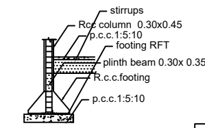
COLUMN DETAILS
