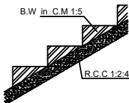
STAIRCASE
