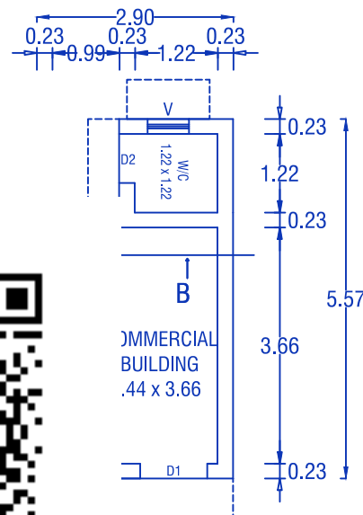
ID FLOOR PLAN
