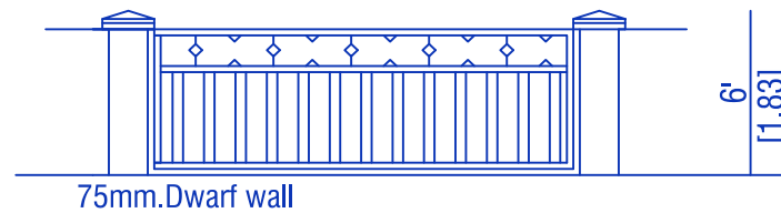
SECTION ON 'AB'
