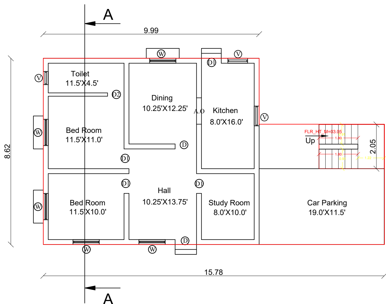
EXG.GROUND FLOOR PLAN
