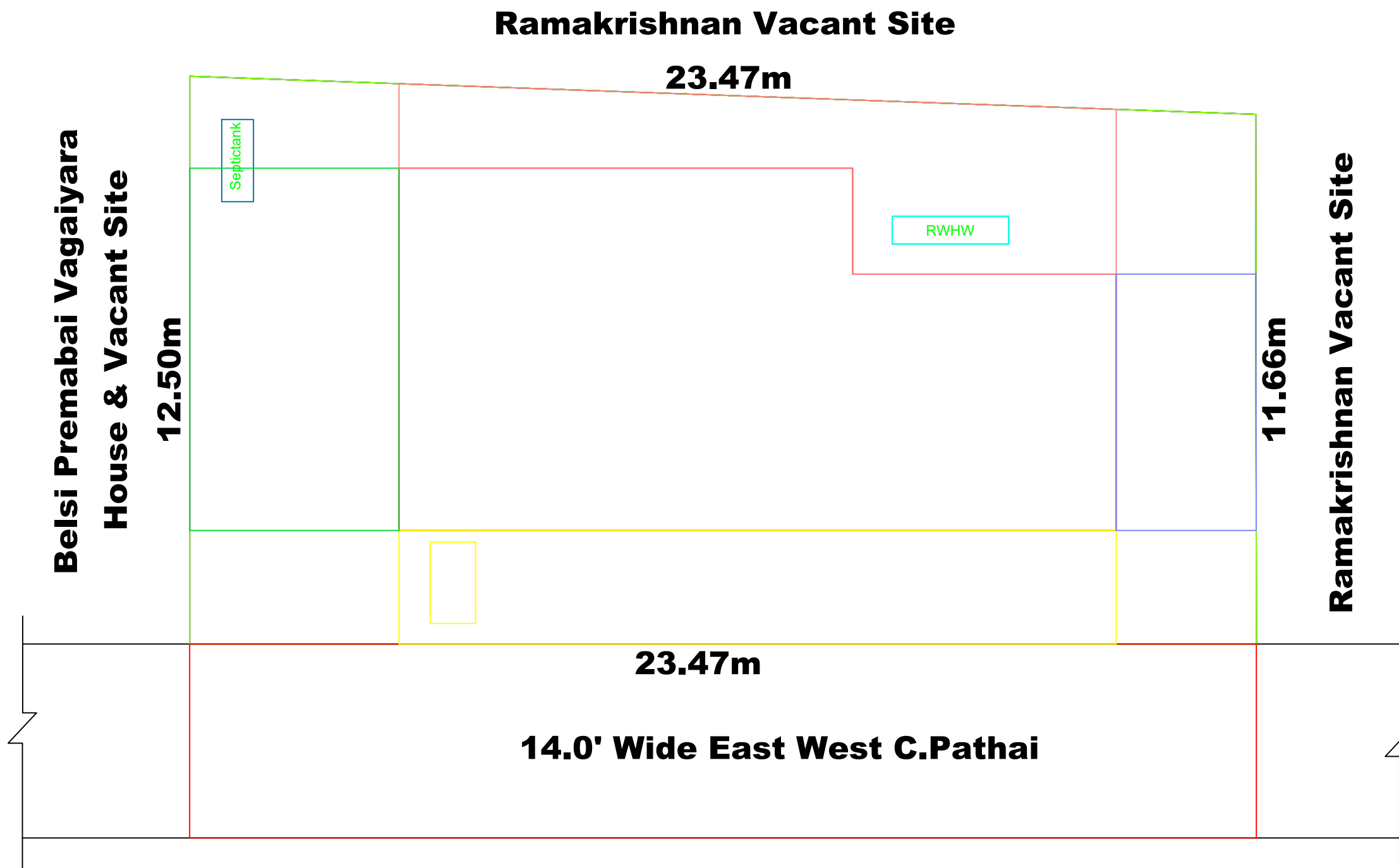
SITE PLAN
