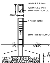
RCC COLUMN DETAILS
