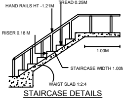
STAIRCASE DETAILS
