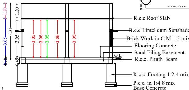
SECTION AA-A
