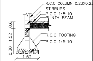
COLOUMN DETAILS
