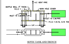
Septic Tank
