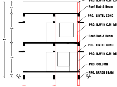
CROSS SECTION ON XX
