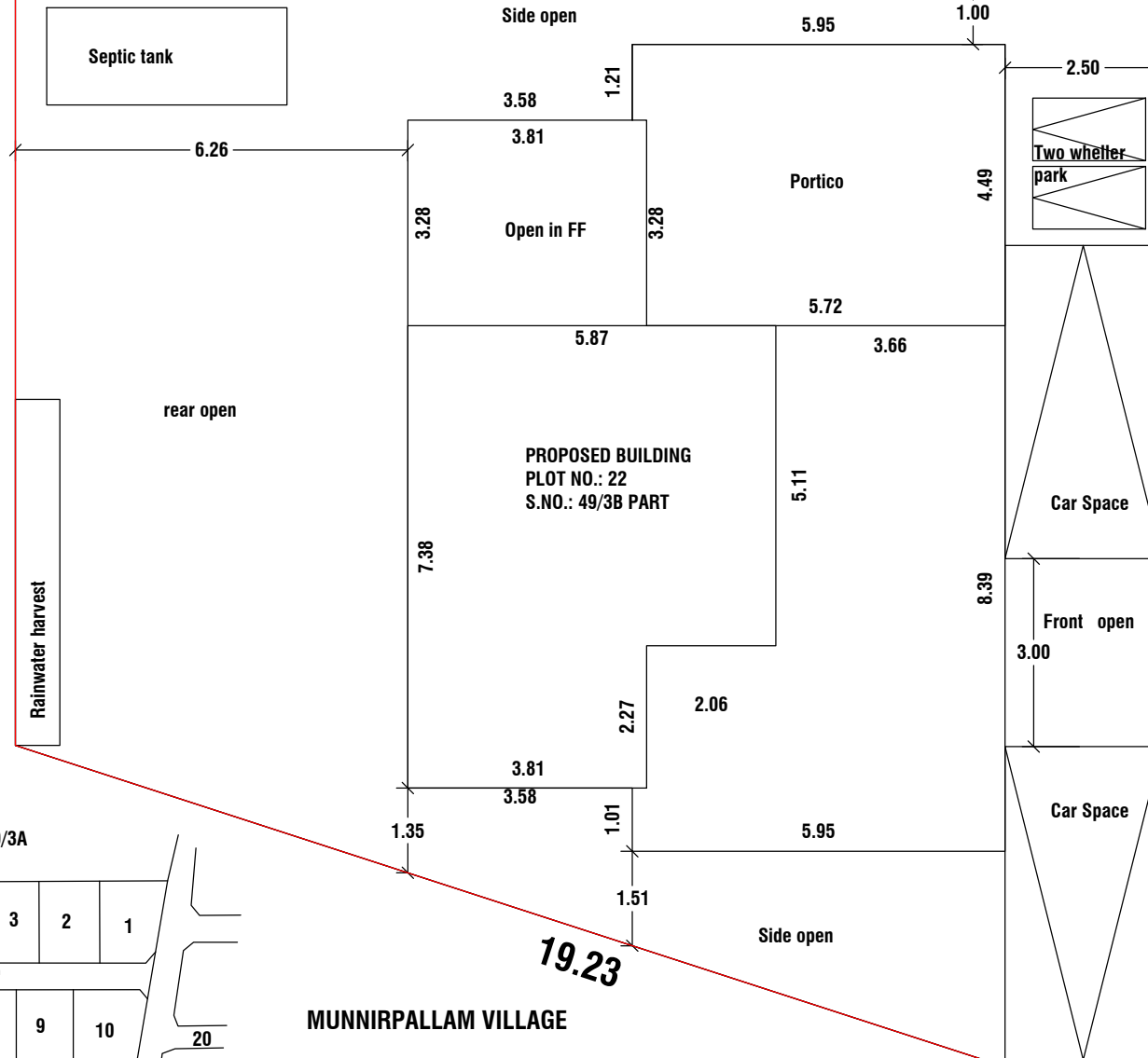
SITE PLAN
