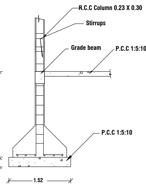
COLUMN DETAIL
