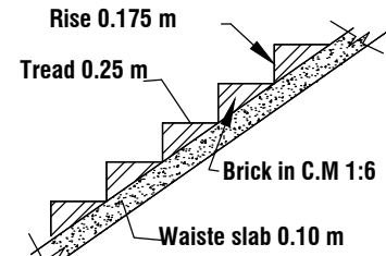
STAIR DETAILS
