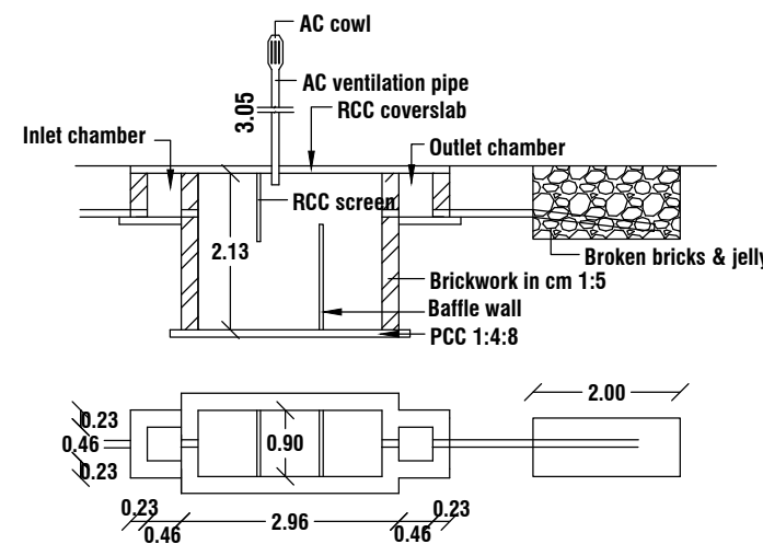
SEPTICTANK DETAILS
