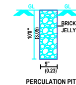
PERCOLATION PIT
