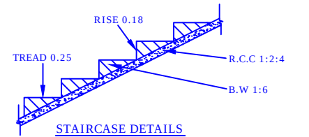
STAIRCASE DETAILS
