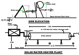
SOLAR WATER HEATER PLANT
