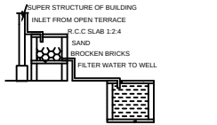
RAINWATER HARVESTING
