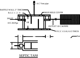
SEPTIC TANK
