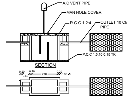
PLAN OF SEPTIC TANK & TRENCH
