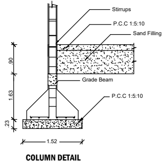
COLUMN DETAIL
