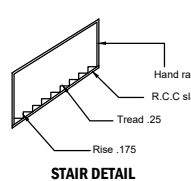
STAIR DETAIL
