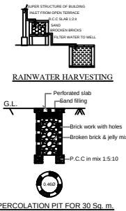
RAINWATER HARVESTING PERCOLATION PIT FOR 30 Sq. m. (NOT FOR SCALE)
