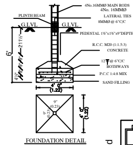
FOUNDATION DETAIL
