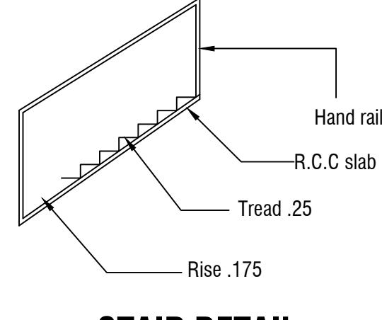
STAIR DETAIL
