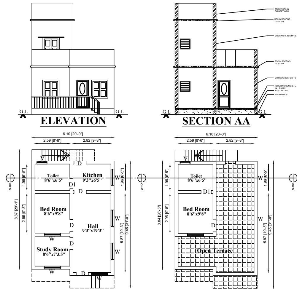
EX.GROUND FLOOR PLAN • PRO.FIRST FLOOR PLAN
