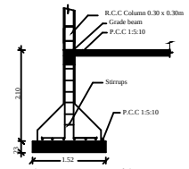
Column Detail
