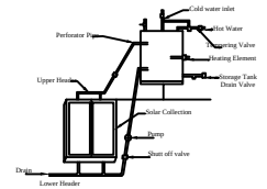
Details Of Solar Water Heater (NTS)
