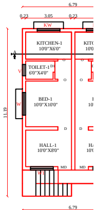
GROUND FLOOR
