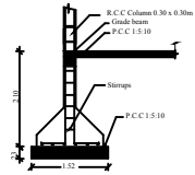
Column Detail
