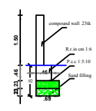
Compound Wall Detail
