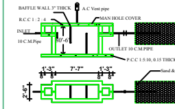
Septic tank and trench
