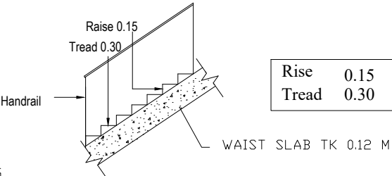
STAIRCASE DETAIL
