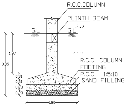
FOUNDATION DETAIL
