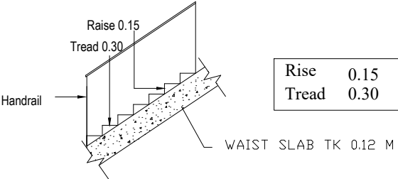
STAIRCASE DETAIL
