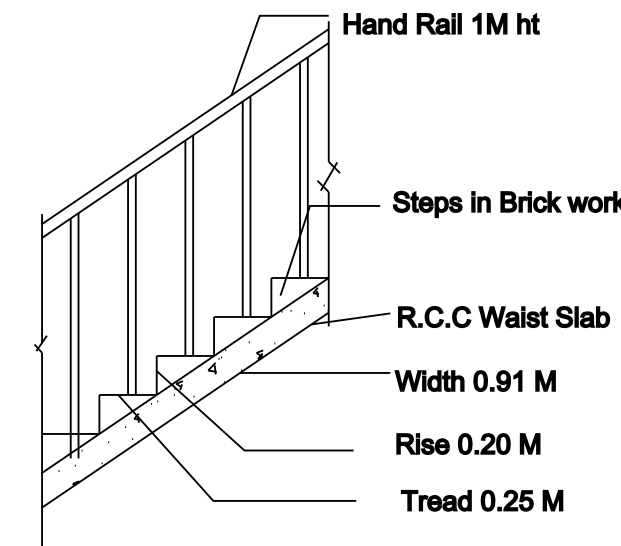
STAIRCASE DETAILS
