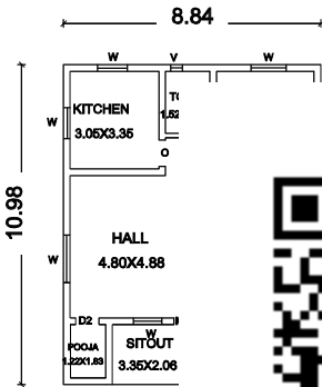
PROPOSED FLOOR
