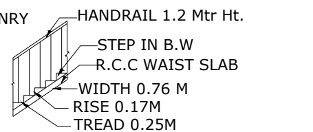
STAIR DETAIL
