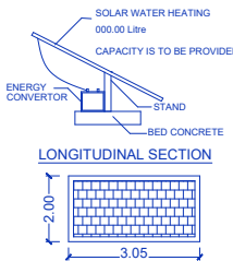
SOLAR SYSTEM
