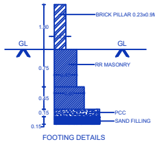
FOOTING DETAILS
