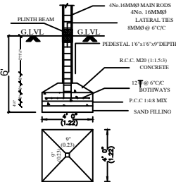
FOUNDATION DETAIL (SCALE: 1:50)
