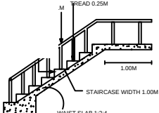
STAIRCASE DETAILS
