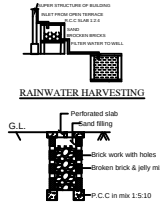
RAINWATER HARVESTING (NOT FOR SCALE)
