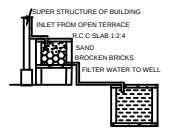
RAINWATER HARVESTING
