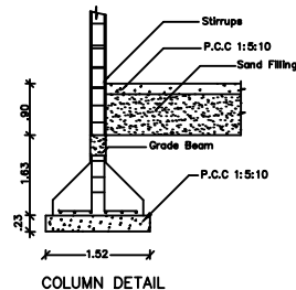
COLUMN DETAIL
