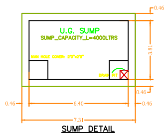
SUMP DETAIL SCALE 1"=4'0"
