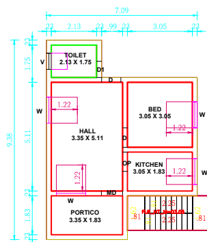
PRO.GROUND FLOOR
