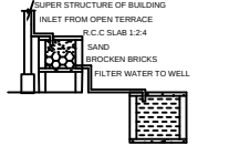
RAINWATER HARVESTING
