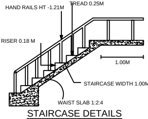
STAIRCASE DETAILS
