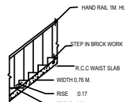
STAIR DETAIL
