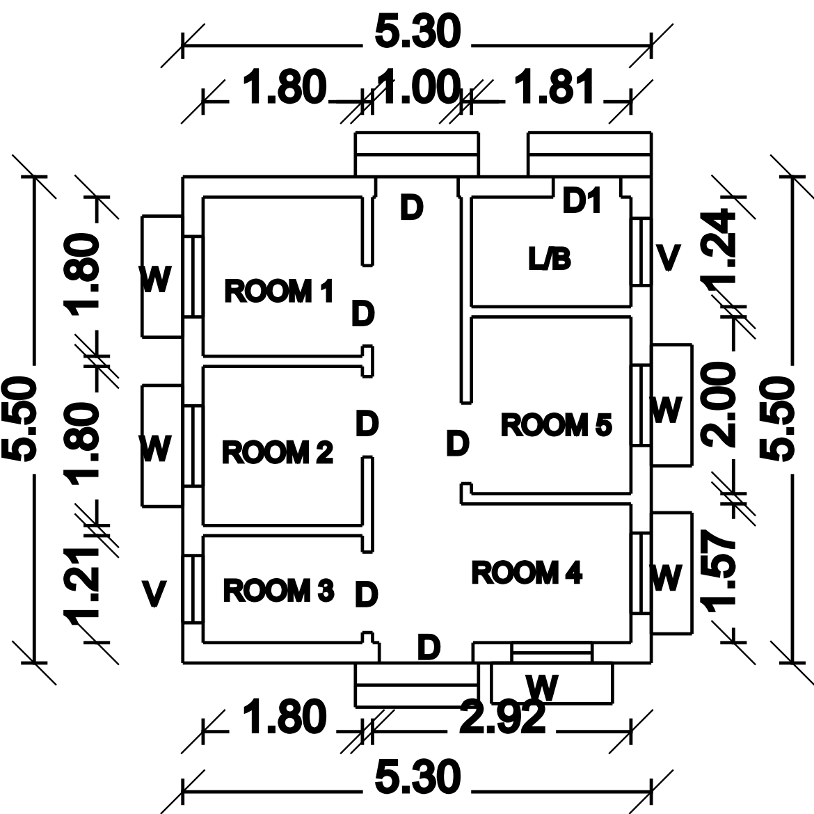
PLAN
