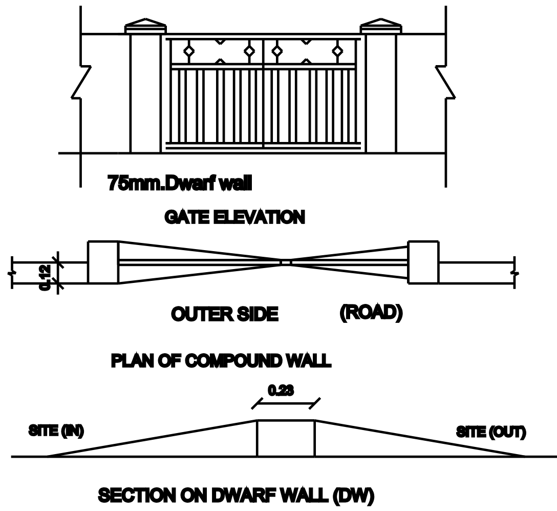
GATE DETAIL
