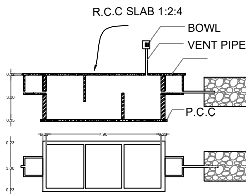
SEPTIC TANK AND TRENCH NTS
