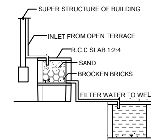
DETAILS OF FILTER BED & WELL NTS
