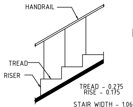
STAIRCASE DETAILS NTS
