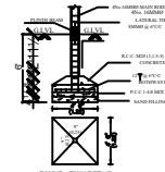
FOUNDATION DETAIL
